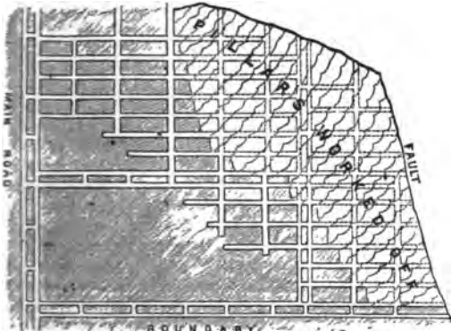
FIG. 9.—Lancashire method of working Coal
