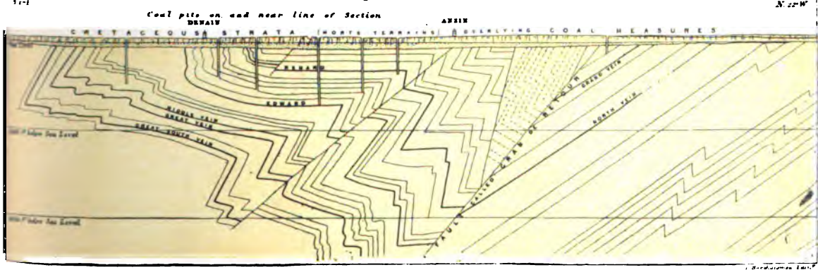
FIG. 4 SECTION ACROSS PART OF THE NORTH OF FRANCE COALFIELD Length about 3 1/4 miles
