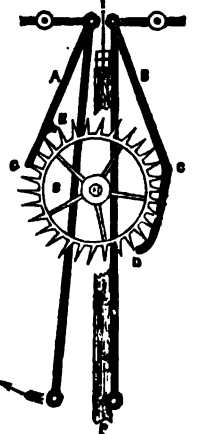
FIG. 18.—Ritchie's Elliptical Escapement.
