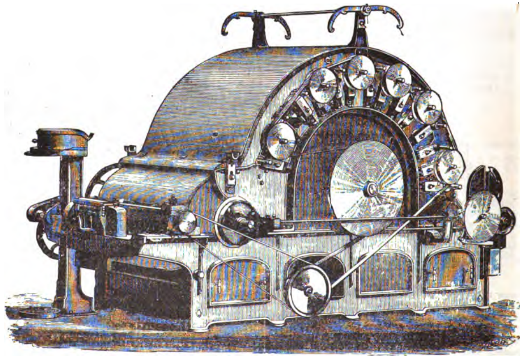
FIG. 6.—Roller and Clearer Carding Machine.
