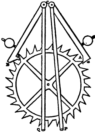
FIG. 10.—Mudge's Gravity Escapement.
