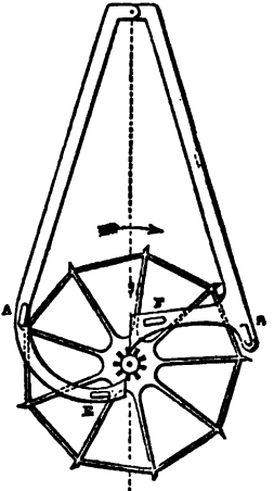
FIG. 11.—Bloxam's Gravity Escapement.
