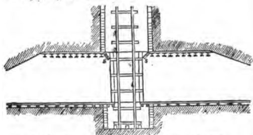
FIG. 5.—Pit eye, Cambolis Colliery—Vertical Section.
