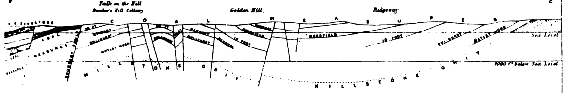
FIG. 3 NORTH STAFFORDSHIRE COALFIELD Length 7 1/2 miles
