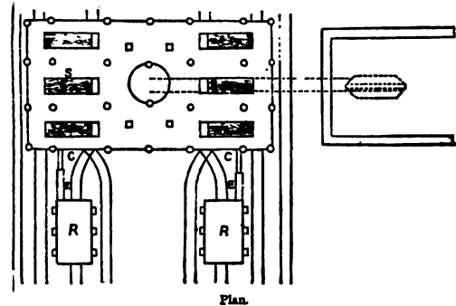
FIG. 25.—Surface arrangements, Pemberton Pit, Wigan.
