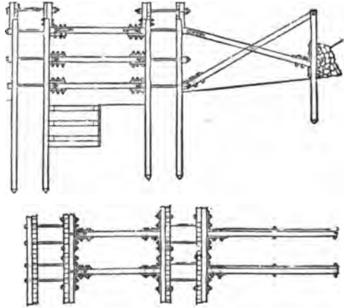
FIG. 2.—Coffer-dam used at Thames Embankment.
