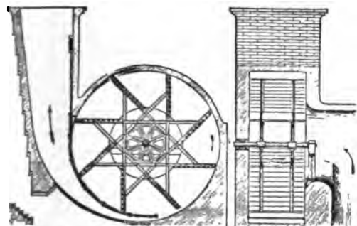
FIG. 17.—Guibal's Fan.
