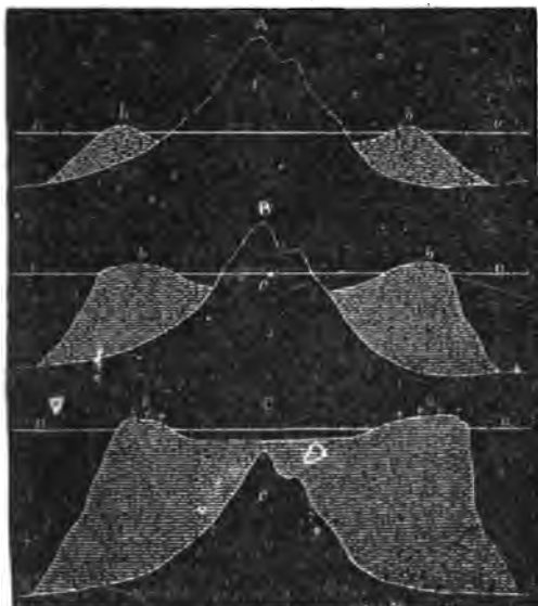
FIG. 10. —Diagrams illustrating the mode of Formation of the different kinds of Coral-reefs.
