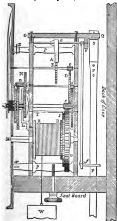
FIG. 1.—Section of House Clock.
