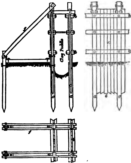
FIG. 1.—Coffer-dam for Soft Bottom.
