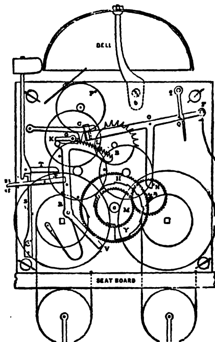
FIG. 15.—Front view of Common English House Clock.
