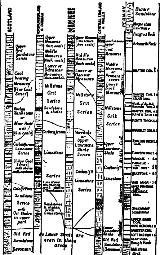
FIG. 1.—Succession of Carboniferous Strata. the index of strata issued by the Geological Survey. The
