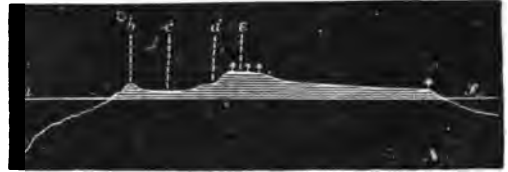
FIG. 9.—Section of Keeling Atoll. (After Darwin.)
