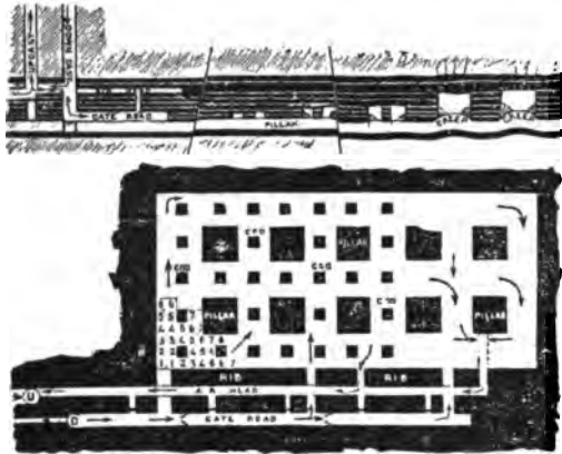
FIG. 11.—South Staffordshire method of working Thick Coal.
