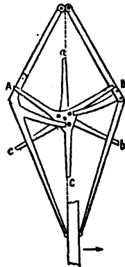
FIG. 13.—Double Three-legged Escapement.
