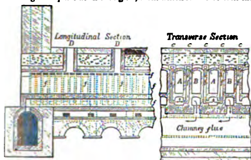
Coppée's Coke Oven.
