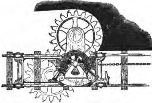
FIG. 14.—Winstanly & Barker's Coal-cutting Machine—Plan.
