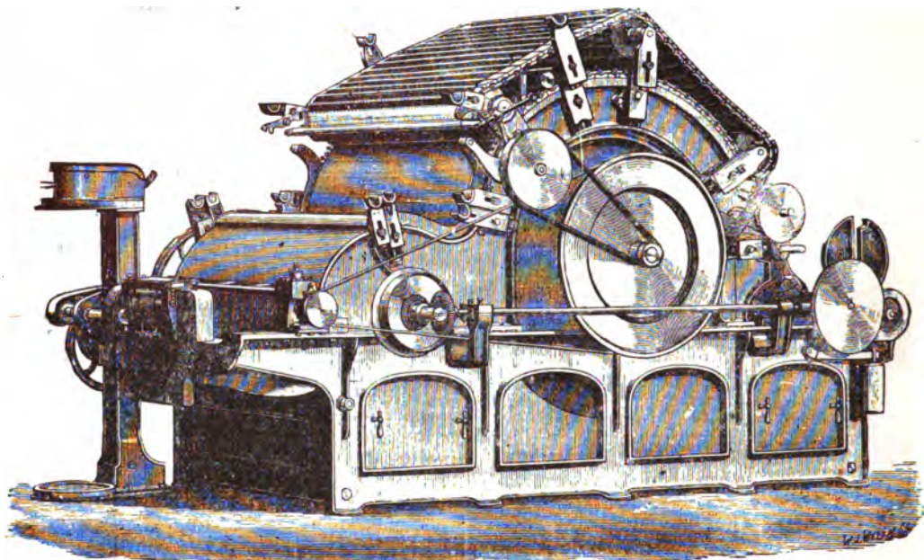
FIG. 5.—Self-stripping Flat Carding Machine.
