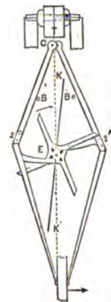
FIG. 12. Four-Legged Gravity Escapement.
