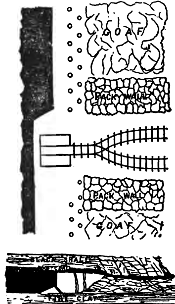
FIG. 12.—Long-wall working-face—Plan and Section.
