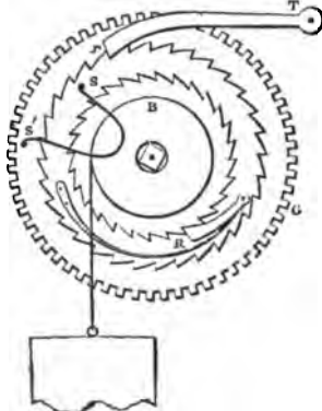
FIG. 14.—Harrison's Going-Ratchet.
