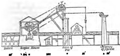
FIG. 22.—Elevation.
