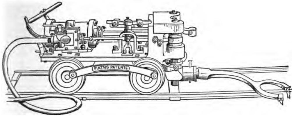
FIG. 13.—Firth's Coal-cutting Machine.
