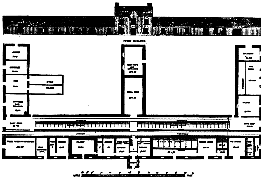
Elevation and Plan of Dairy Farm-steading.
