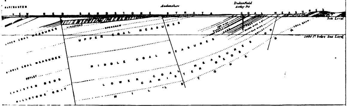
FIG. 2 SOUTH PART OF THE LANCASHIRE COALFIELD Length 7 1/2 miles
