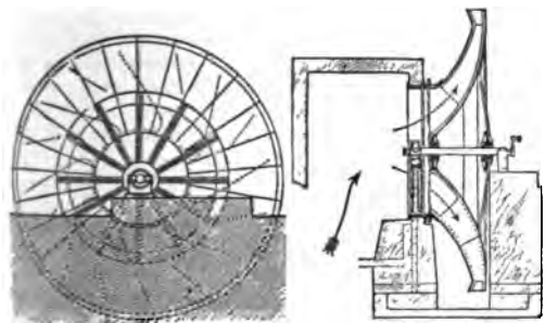
FIG. 18.—Waddle's Fan.
