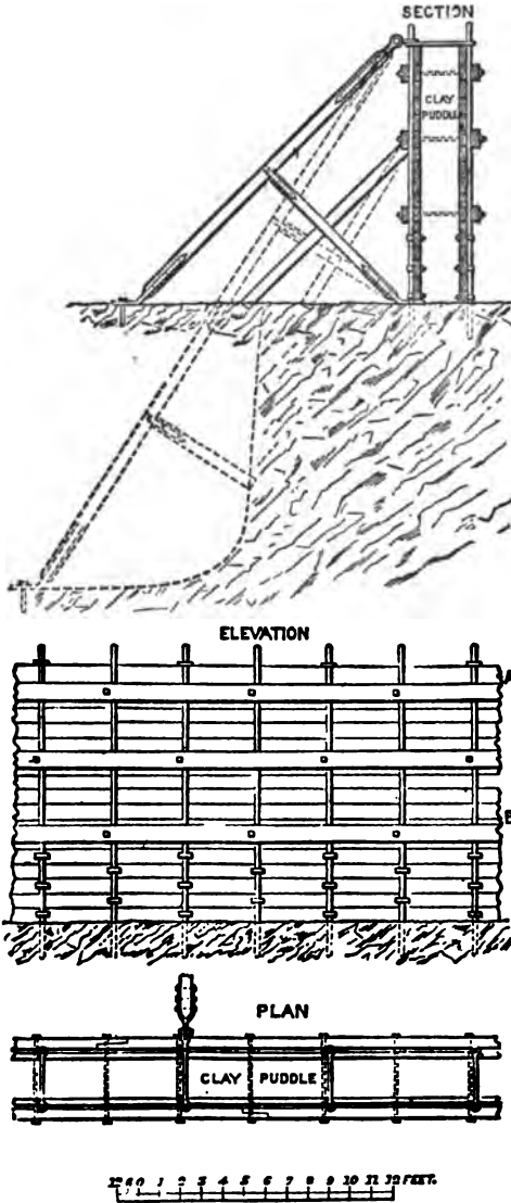
FIG. 8.—Cofferdam for Hard Bottom.
