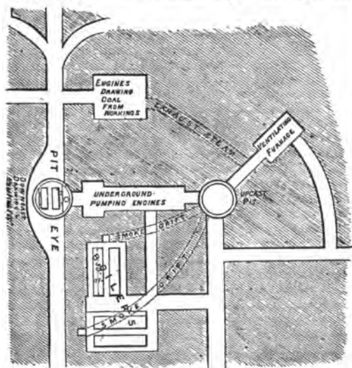
FIG. 6.—Pit bottom arrangements, Cambolis Colliery
