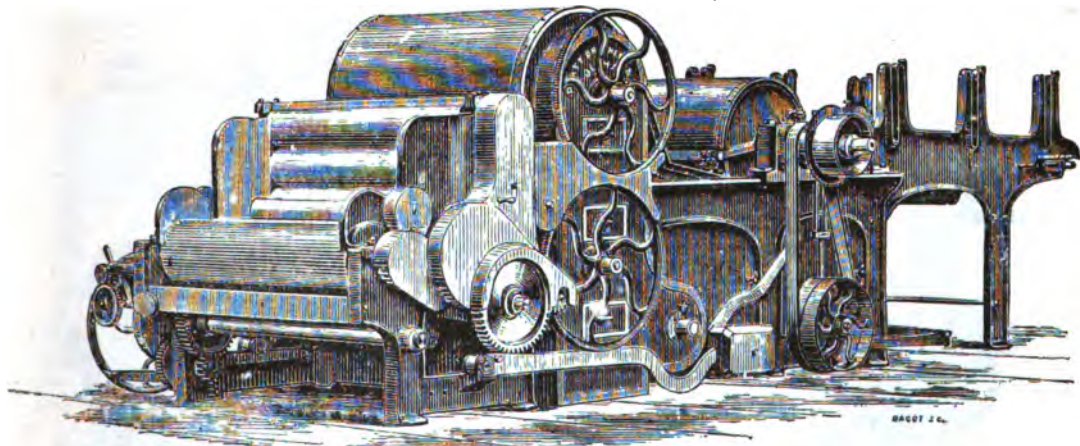
FIG. 4.—Single Scutcher and Lap Machine.
