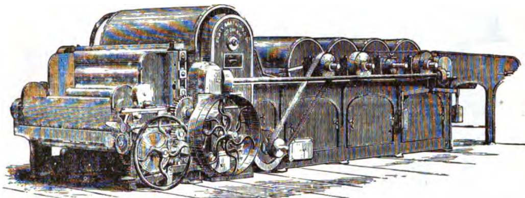
FIG. 3.—Three-cylinder Opener, Beater, and Lap Machine.
