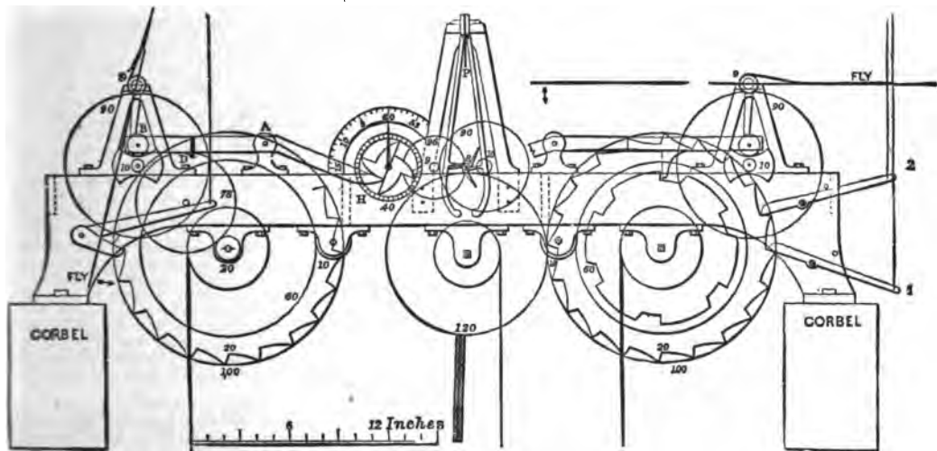
FIG. 22.—Front view of Turret Quarter Clock.
