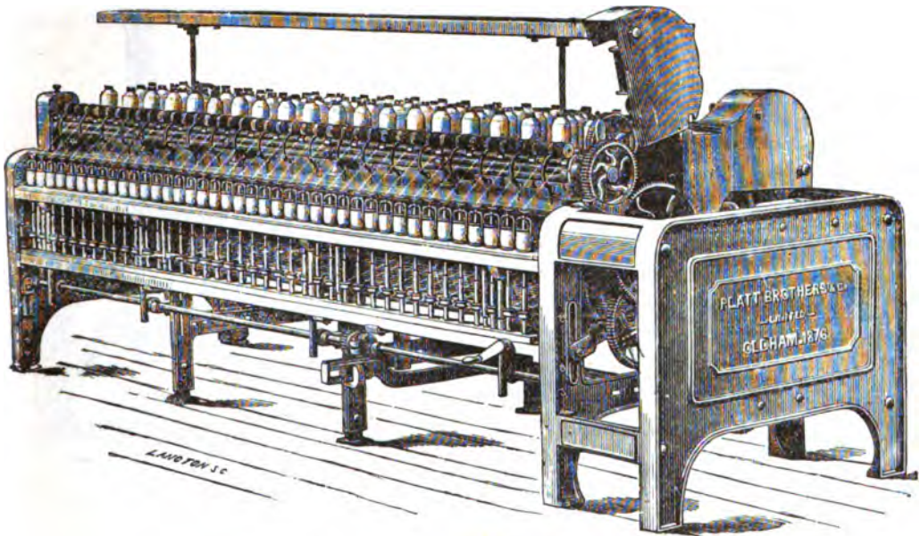
FIG. 11.—Throstle with Spindles and Flyers.
